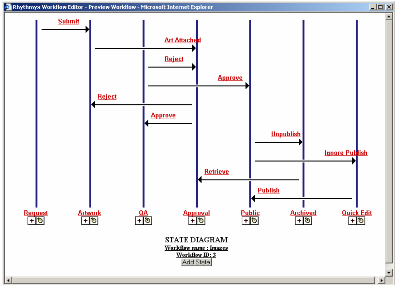
Figure 22: Images Workflow
